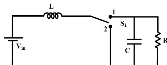
Figure 2: BUCK CONVERTER
