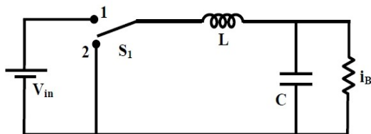
Figure 4 BUCK-BOOST CONVERTER
