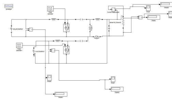
Figure 9: Simulation Design Model
