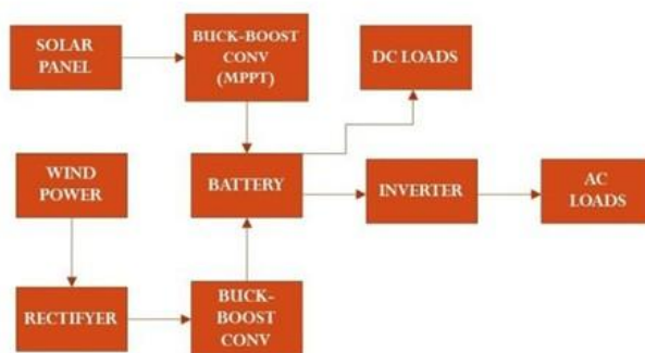
Figure 1: Block diagram of hybrid system
