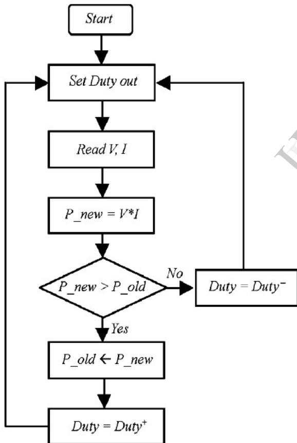
Figure 8: FLOW CHART FOR P & O
