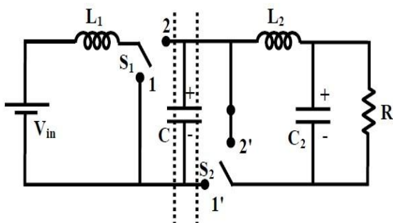
Figure 5: CUK CONVERTER
