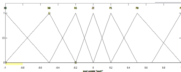
Fig.5.Membership functions of input \epsilon
