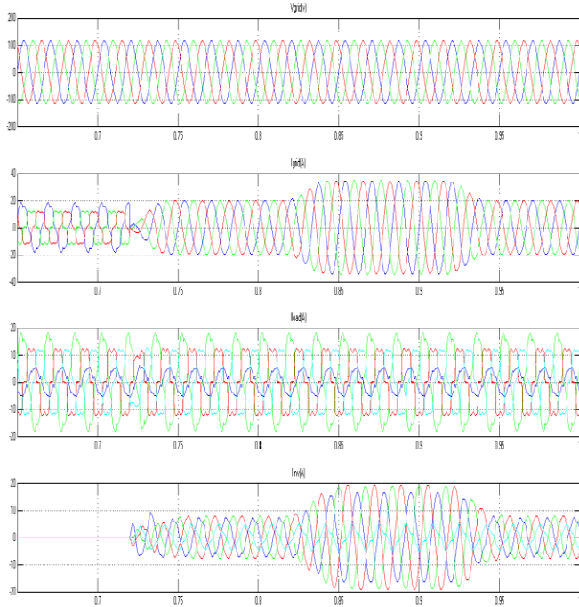
Fig.7. simulation results:(a)grid voltages, (b) grid currents, (c) load currents,(d) inverter currents
