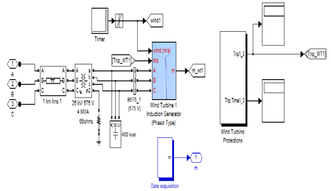
Fig. 2. simulink diagram of wind farm.
