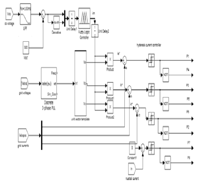
Fig. 3. Representation of grid interfacing inverter control
