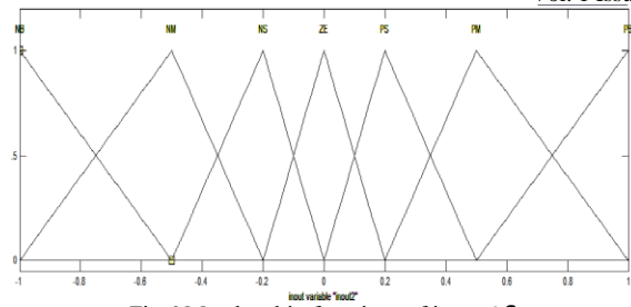
Fig.6.Membership functions of input \Delta\epsilon
