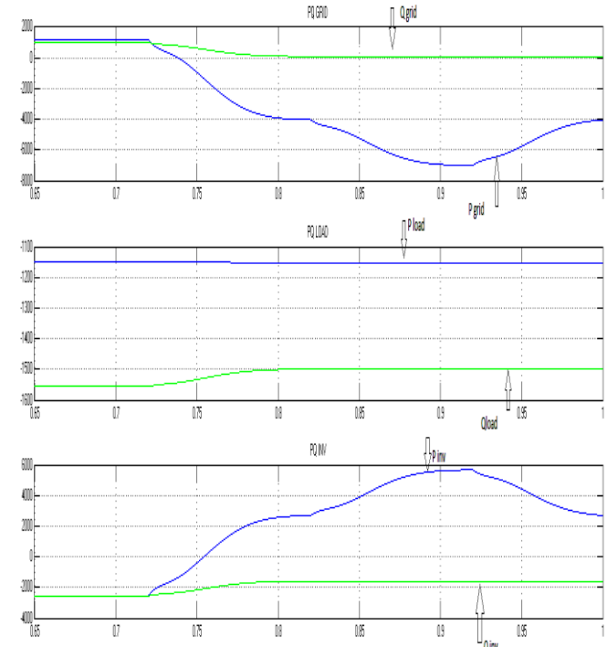
Fig.9.simulation results: (a) PQ grid, (b) PQ load, (c) PQ inverter using PI controller
