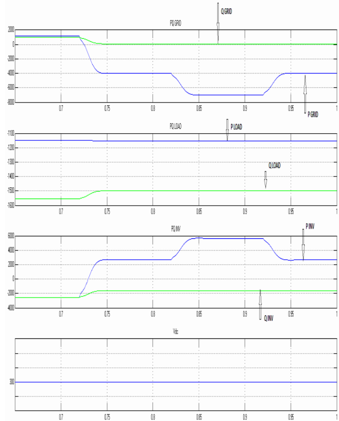
Fig.8.simulation results: (a) PQ grid, (b) PQ load, (c) PQ inverter, (d) dc link voltage using fuzzy controller
