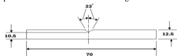
Fig.2.1 Length of the specimen diemensions according to ASTM diemensions
