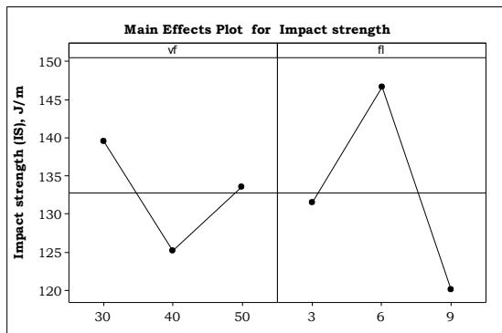
Fig.2.7. Effect of control factors on Impact strength (IS)
