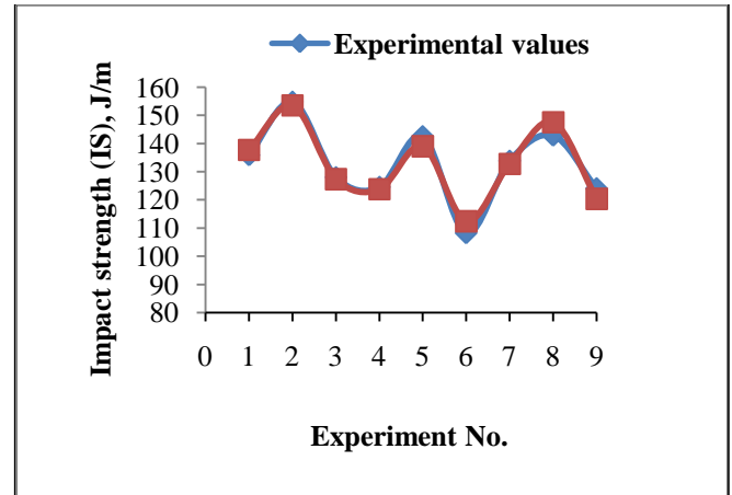
Fig 2.8. Variation of Impact strength with respect to Experiment no.
