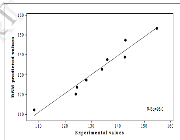
Fig.2.5 Comparison plot for Impact strength
