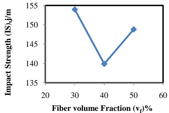
Fig.2.5. Variation of Impact strength with respect to Fiber volume fraction ( v_f ) %
