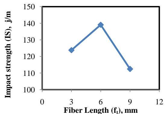
Fig.2.6. Variation of Impact strength with respect to Fiber Length ( f_l ), mm
