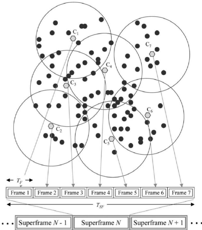
Fig. 1 MH-TRACE clustering and medium access for a portion of an actual distribution of mobile nodes. Nodes C through C are cluster head nodes.
