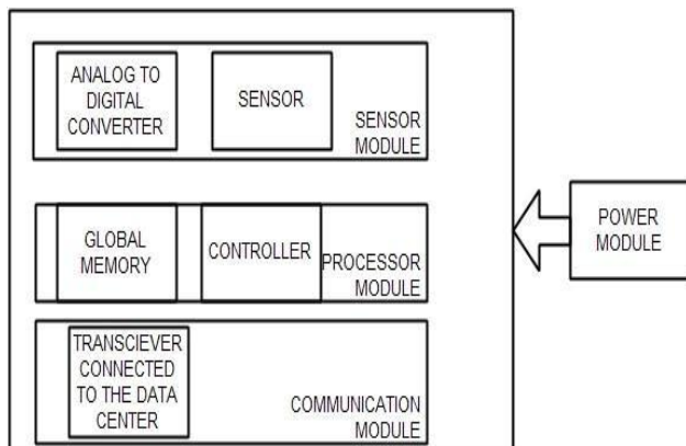
Fig. 3. Sensor Node of the Smart Agriculture Solution
