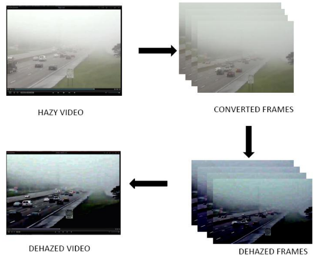
Fig. 6: Dehazing Video
