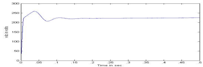
Fig. 7(e) DC capacitor voltage
