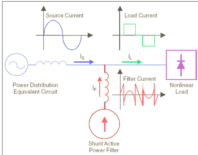
Fig. 1: Basic Compensation Principle
