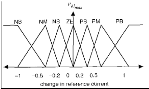
Fig. 6: Output Normalized Membership Function
