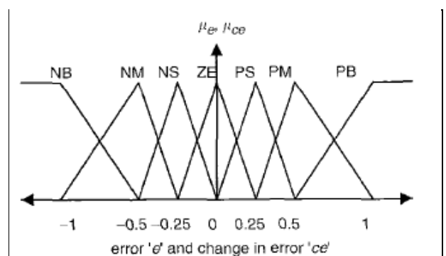
Fig. 5: Input Normalized Membership Function
