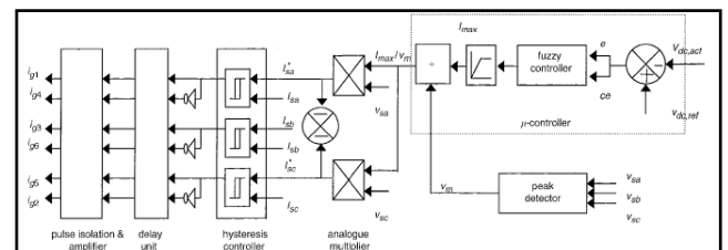
Fig.3: Fuzzy Control scheme
