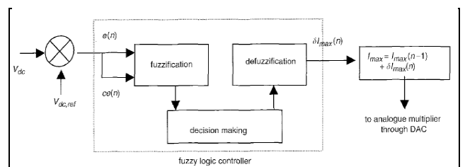
Fig. 4: Internal Structure of Fuzzy controller
