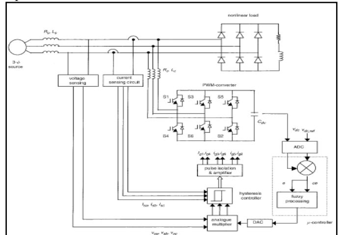
Fig.2: Schematic Diagram of Closed Loop Fuzzy Logic Controlled Shunt Active Power Filter
