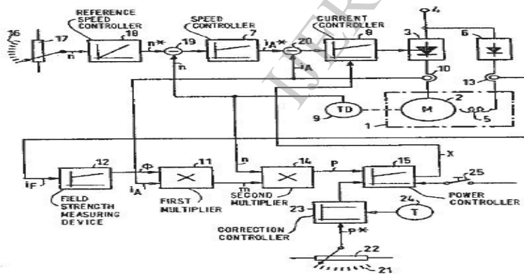
Figure no. 2 SPED CONTROLLER WITH CUURENT CONTROLLER
