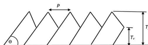
Fig. 4. Segmented chip morphology parameters
