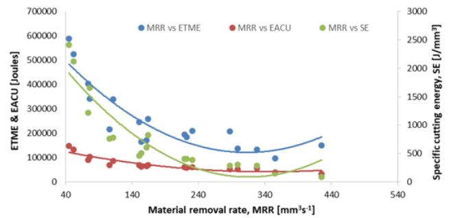
Fig. 6. Material removal rate, MRR vs specific cutting energy, SE
