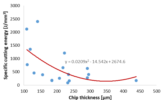
Fig. 11. Variation of specific cutting energy as a function of chip thickness
