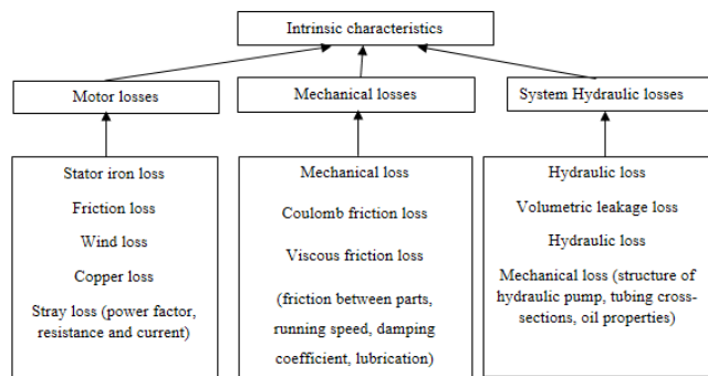
Fig. 1. Intrinsic characteristics and processing conditions which affect energy efficiency on the machine tool, [5]
