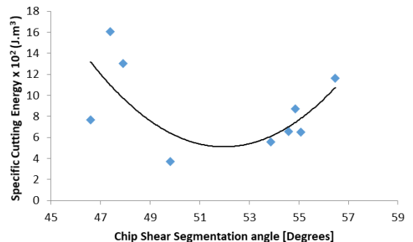
Fig. 9. Variation of specific cutting energy as a function of chip shear segmentation angle
