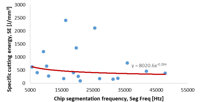
Fig. 8. Variation of specific cutting energy with change in chip shear segmentation frequency
