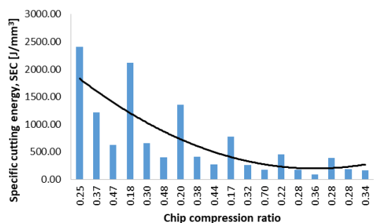
Fig. 12. Variation of specific cutting energy as a function of chip compression ratio
