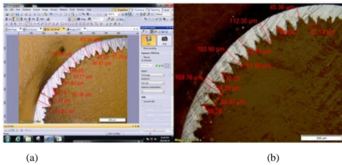
Fig. 5. Chip morphology profile measured parameters (a) image on computer screen – v_c = 50 m/min at f_n = 0.2 mm/rev (b) v_c = 70 m/min at f_n = 0.2 mm/rev
