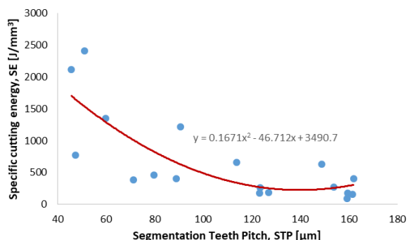
Fig. 10. Variation of specific cutting energy as a function of chip shear segmentation pitch
