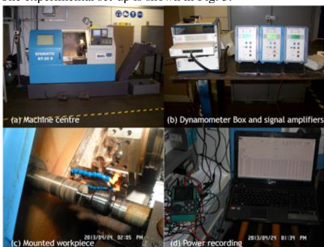
Fig. 3. Experimental set-up
