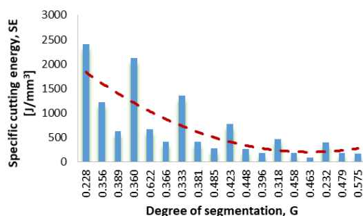
Fig. 13. Variation of specific cutting energy as a function of degree of segmentation
