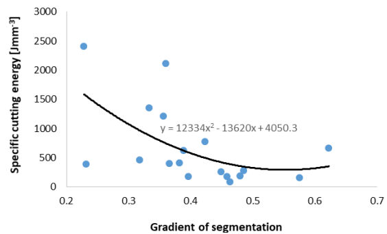
Fig. 7. Variation of specific cutting energy as a function of gradient of segmentation
