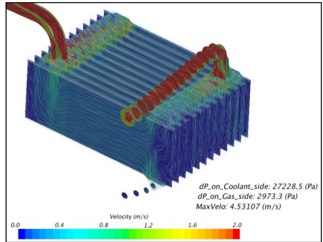
Fig 11. CFD analysis for pressure Drop
