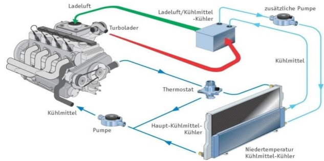
Fig.2 Indirect / Water cooled charge air cooler system
