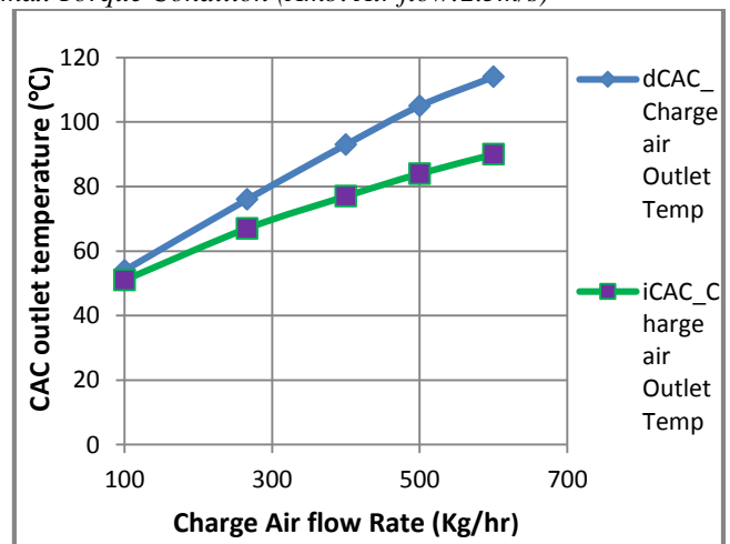
Fig 13. Performance comparison curve (Outlet temp Vs Charge air flow)
