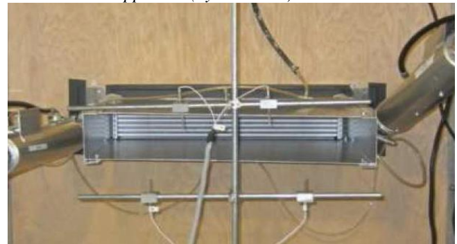
Fig 7. Test Bench set up for dCAC
