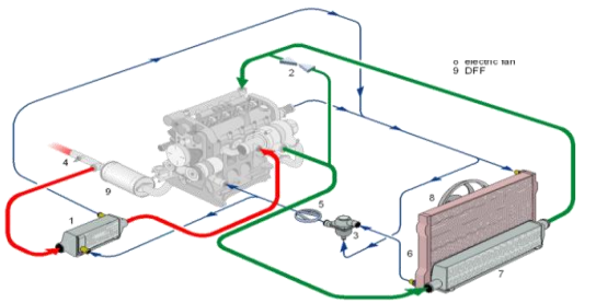
Fig.1 Direct/Air to air charge air cooler system
