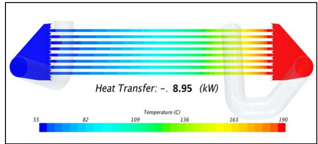
Fig.5 CFD analysis for heat rejection calculation
