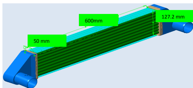
Fig.4 Direct/Air to air charge air cooler
