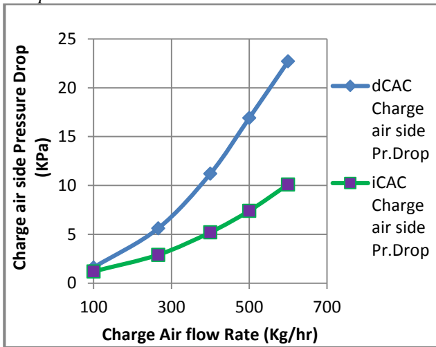
Fig 13. Performance comparison curve (Charge air Pressure Drop Vs Charge air flow)
