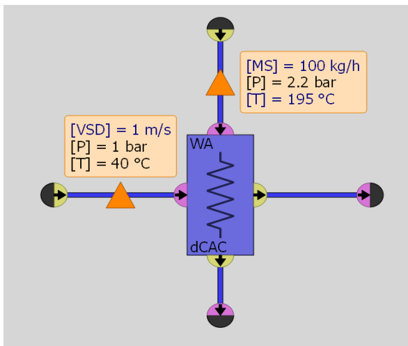
Fig.3 Simulative approach for direct charge air cooler
