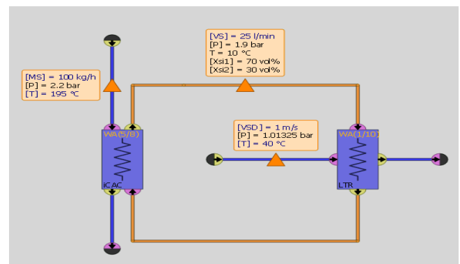
Fig 8. Simulative approach for Indirect charge air cooler
