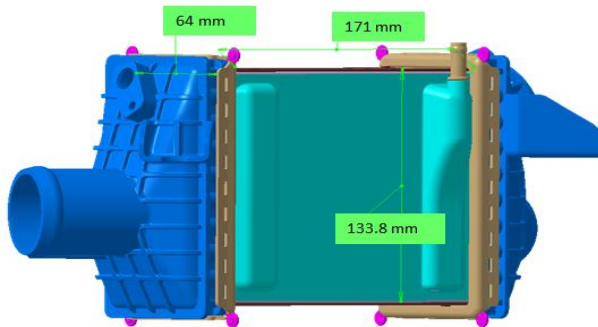
Fig. 9. Indirect charge air cooler
