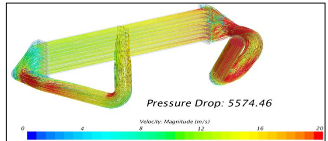
Fig.6 CFD analysis for Pressure Drop calculation
