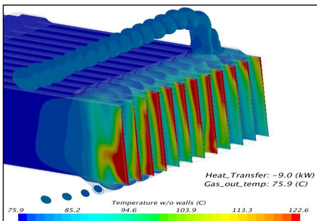
Fig 10. CFD analysis for Heat Rejection
