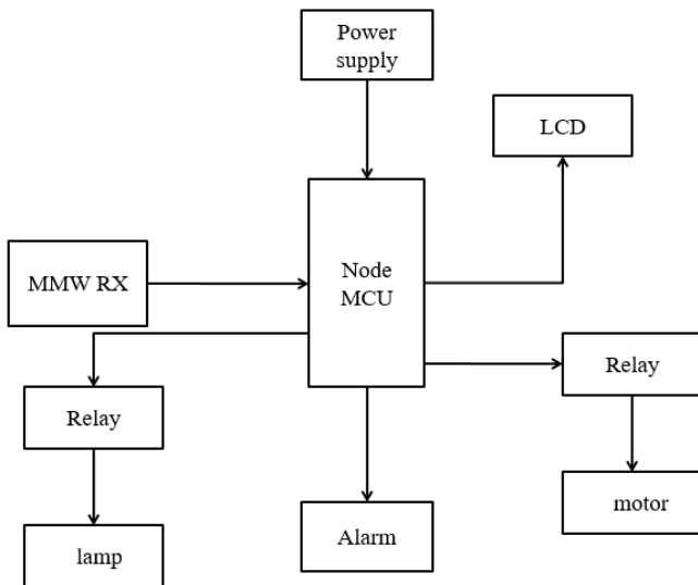
Figure 2 : Receiver block diagram
