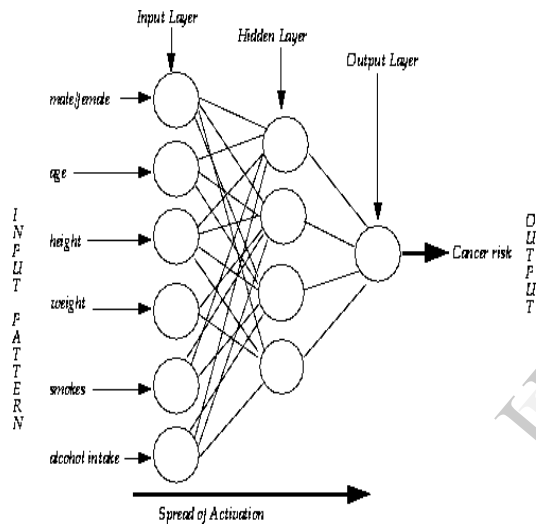
Figure 3.3 Neural networks from Clementine User Guide
