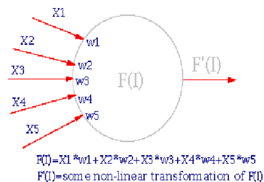
Figure 3.2 Interconnection weight of neural network
